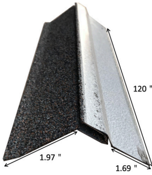
Starter Course
